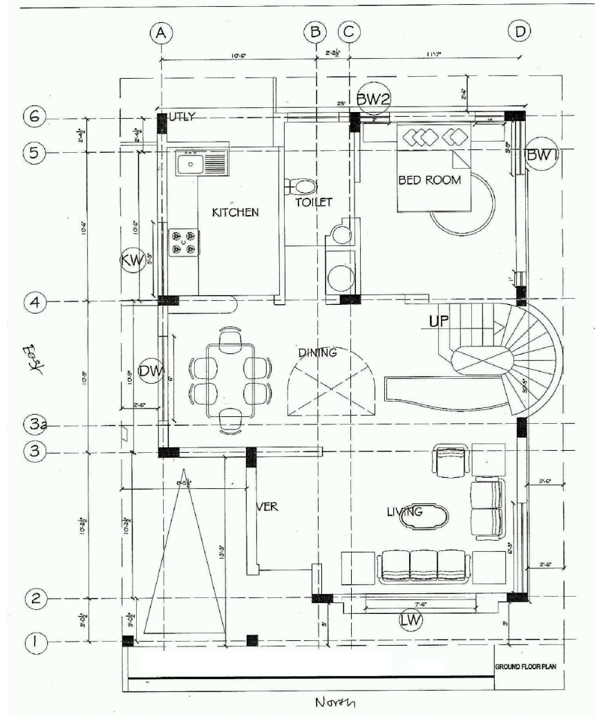
Farm house ground floor plan
