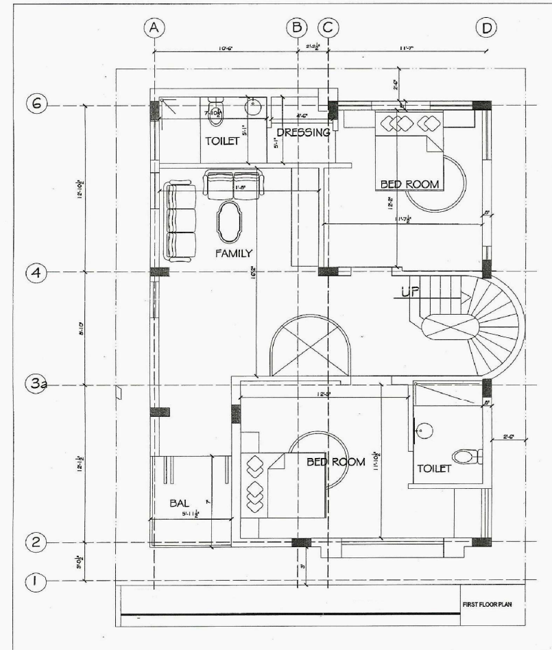
Farm house 1st floor plan
